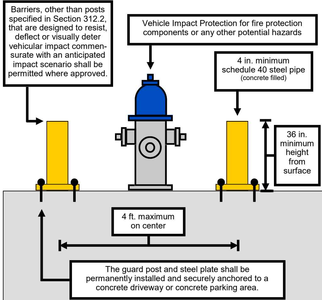
ELEVATION VIEW
